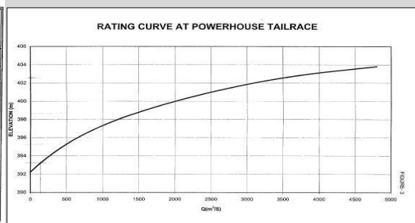
Fig.7- Rating Curve (Typical)
