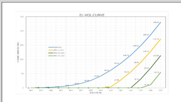
Fig.10-Sedimentation deposition Study (Typical)
