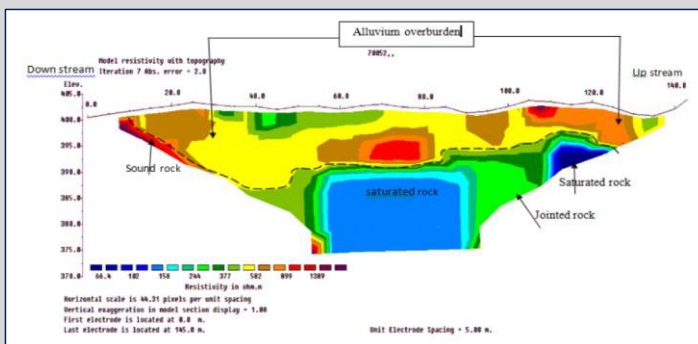
Fig.11 shows the ground profile from ERT.
