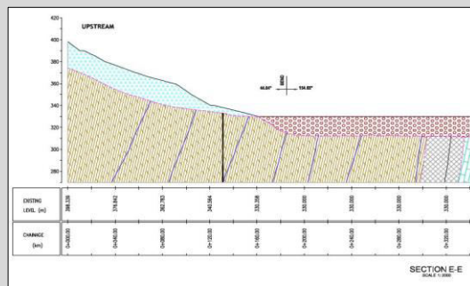
Fig.14. Typical Geological Section.
